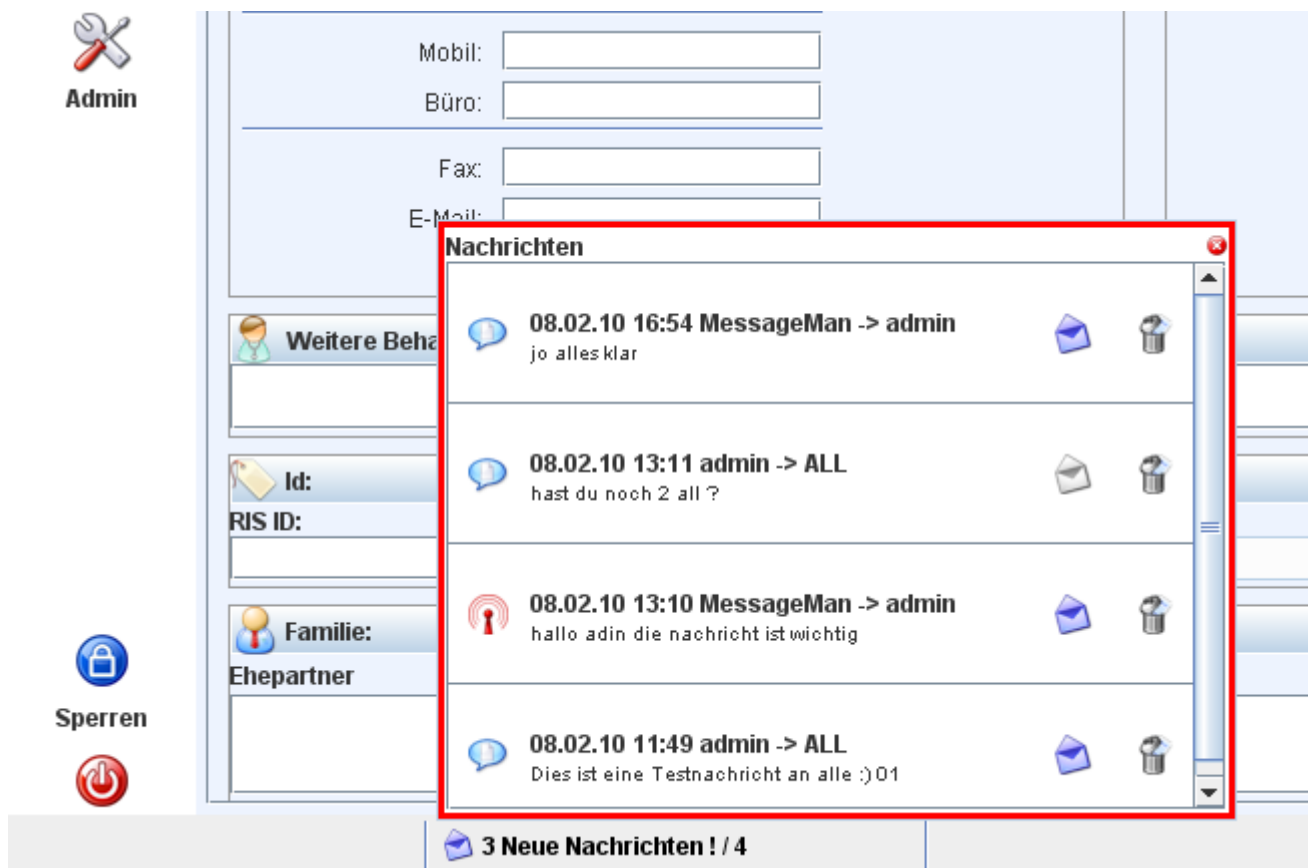
Abb. 1: Message Board
